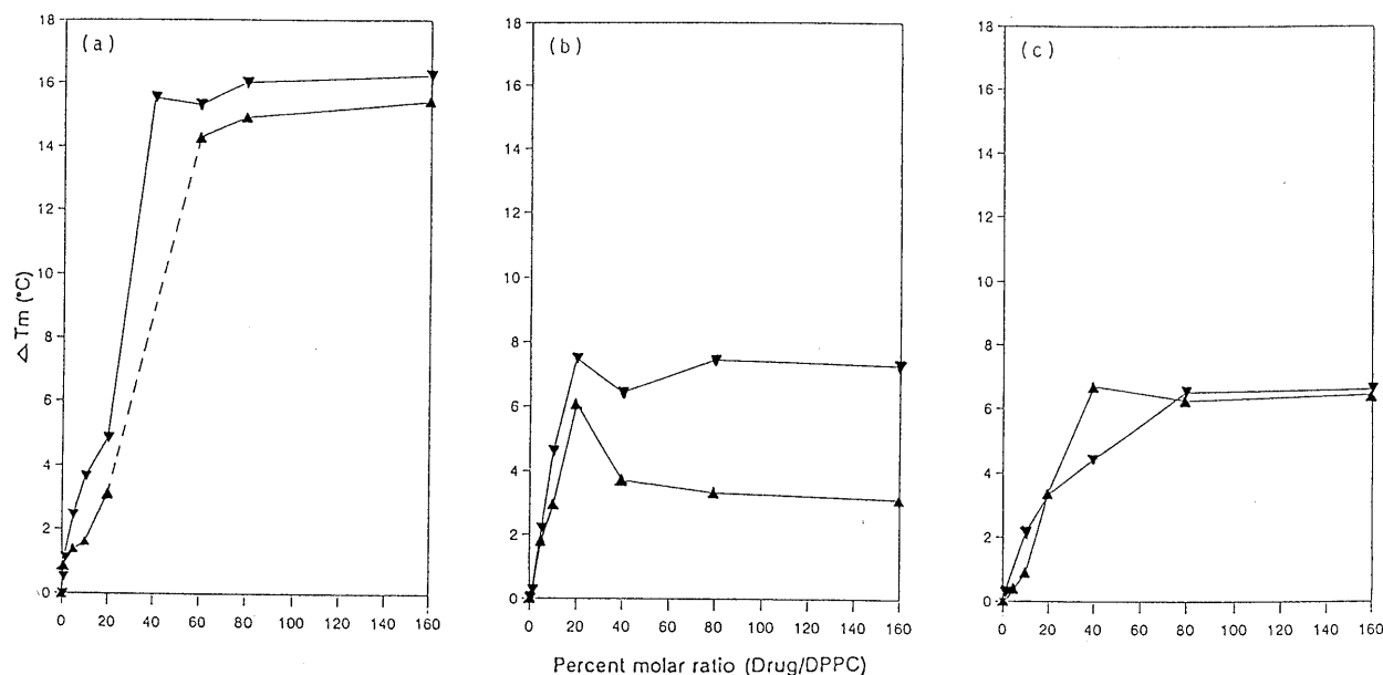
Fig. 5. Variation of the Change in Transition Temperature ( \Delta T_m ) as a Function of (a) Halofantrine/DPPC Molar Ratio (%) at pH 7.4 [▼] and pH 11.0 [▲]; (b) Mefloquine/DPPC Molar Ratio (%) at pH 7.4 [▼] and pH 10.0 [▲] and (c) Quinine/DPPC Molar Ratio (%) at pH 6.0 [▼] and pH 10.0 [▲]
