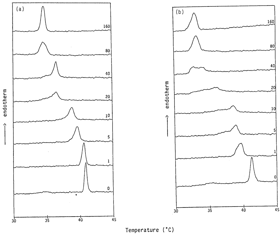
Fig. 4. DSC Curves of DPPC Liposomes Containing 0% to 160% Molar Ratio of Quinine/DPPC Obtained at (a) pH 6.0 and (b) pH 10.0
