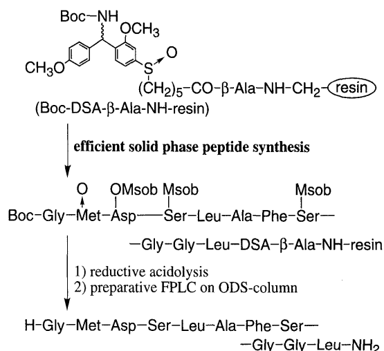
Chart 10. Synthesis of Buccalin
