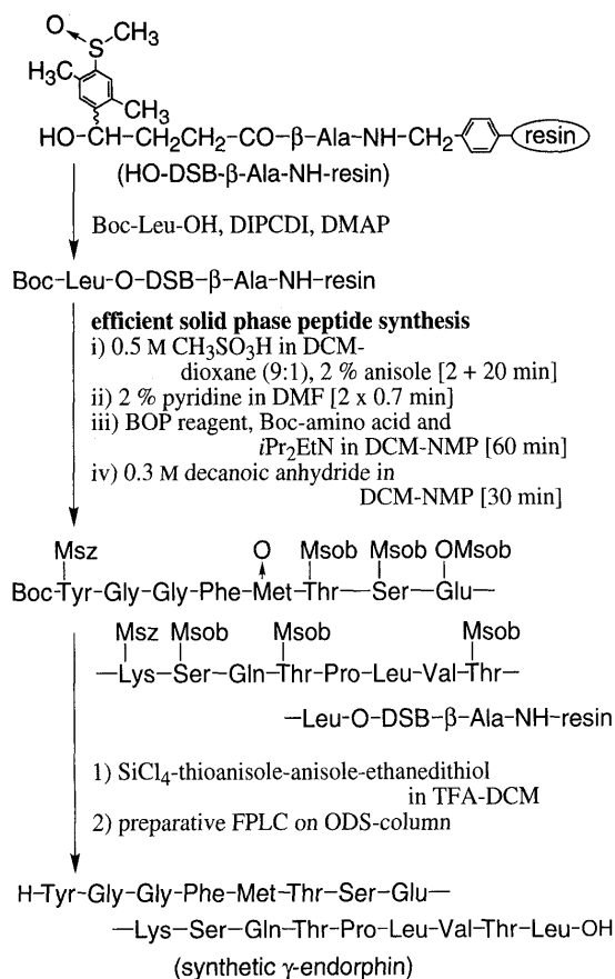
Chart 9. Synthesis of γ-Endorphin
