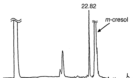
Fig. 3. HPLC Elution Pattern of Crude Buccalin Conditions: column, YMC AM302 (ODS) (4.6 × 150 mm); eluent, MeCN 10%–60% (30 min) in 0.1% TFA; flow rate, 0.7 ml/min; O.D., 230 nm.
