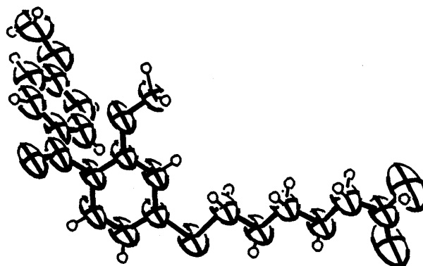
Fig. 4. X-Ray Crystal Structure of 4-(4-Methoxybenzoyl)-3-methoxyphenylthio-6-hexanoic Acid
