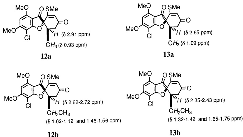
Fig. 2. ^1\text{H-NMR} (500 MHz) Data for Thiogriseofulvins ( 12a, b , 13a, b )
