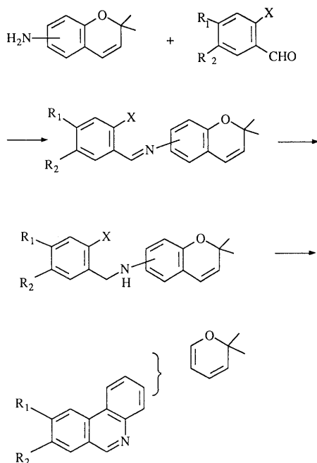
Chart 1. Synthesis of Pyranophenanthridines
