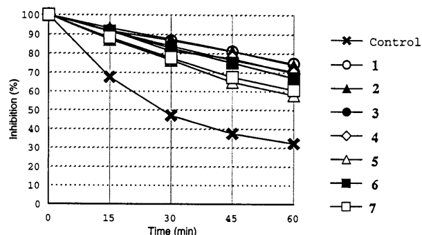
Fig. 2a. Effects of Compounds 1—7 on the Photo-Oxidation of Vitamin \text{B}_6
