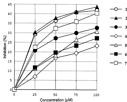
Fig. 1. Effects of Compounds 1—7 on Superoxide Anion
