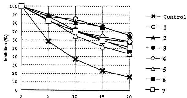
Fig. 2b. Effects of Compounds 1—7 on the Photo-Oxidation of Vitamin \text{K}_1
