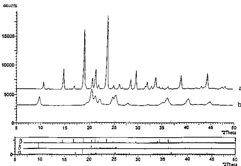
Fig. 2. Powder X-Ray Diffraction Patterns
