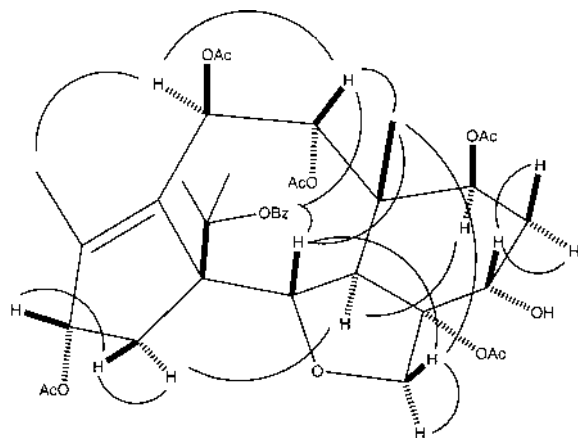
Fig. 1. NOESY Correlation of Taxumairol G ( 1 )
