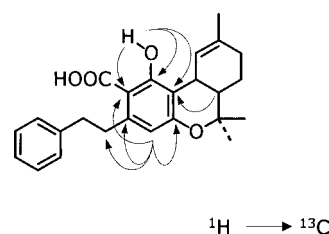
Fig. 2. HMBC Correlations for Perrottetinenic Acid ( 2 )
