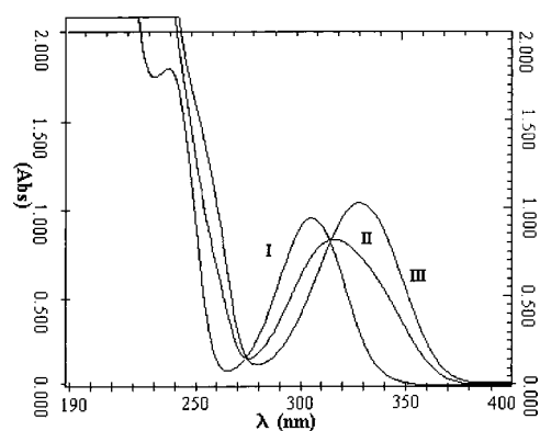
Fig. 4. Absorption Spectra of 2,3-DHBA ( T_L=3.0 \times 10^{-4} \text{ mol} \cdot \text{l}^{-1} ) I: \text{pH}=4.97 ; II: \text{pH}=10.17 ; III: \text{pH}=12.50 .
