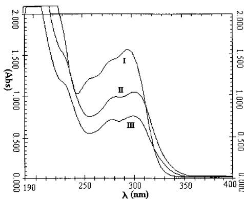
Fig. 9. Absorption Spectra of Y(III) Complexes of 3,4-DHBA in 0.1 M NaClO 4 at 25 °C (pH=9.0)
