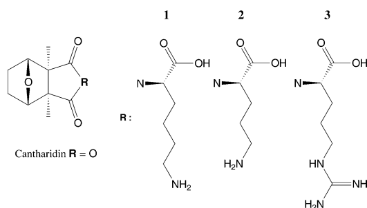
Fig. 2. Structures of 1 , 2 , and 3
