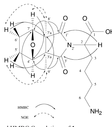
Fig. 1. NOE and HMBC Correlations of 1
