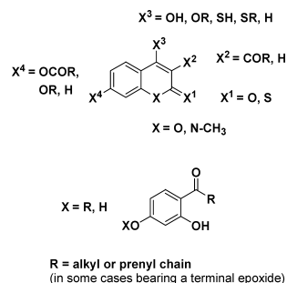
Fig. 2. Isosters and Chemical Modifications of Coumarin and Acetophenone
