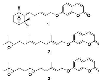
Fig. 1. Meroterpenoid Inhibitors for SHC
