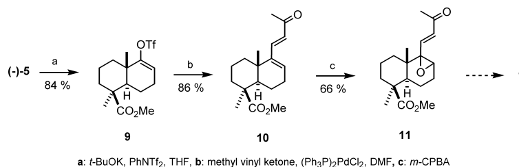
Chart 2. Synthetic Route of 1 from (–)- 5 using Heck Reaction as a Key Step
