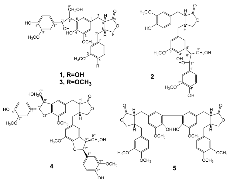
Fig. 1. Chemical Structures of Compounds 1–5 Isolated from A. lappa
