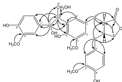
Fig. 2. Selected HMBC Correlations of Compound 1
