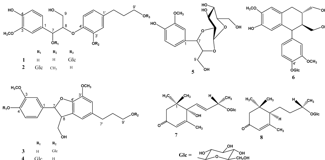
Fig. 1. Structures of 1–8
