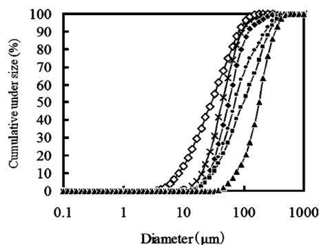
Fig. 3. Particle Size Distribution of Composite Particles Prepared with Varying Solution Concentration
