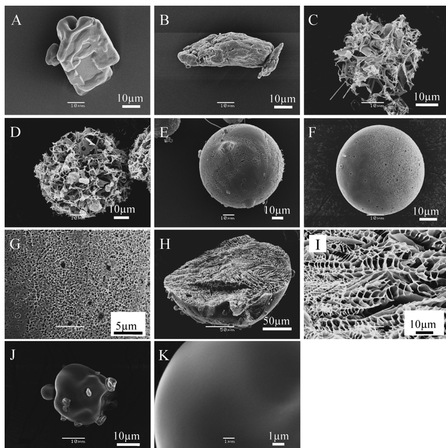
Fig. 2. SEM Photographs of Bulk Materials and SFD Composite Particles with Varying Solution Concentrations
