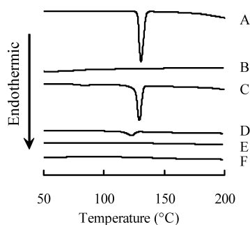
Fig. 7. DSC Profiles of Samples
