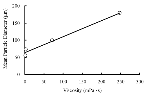
Fig. 4. Relationship between Particle Diameter and Solution Viscosity
