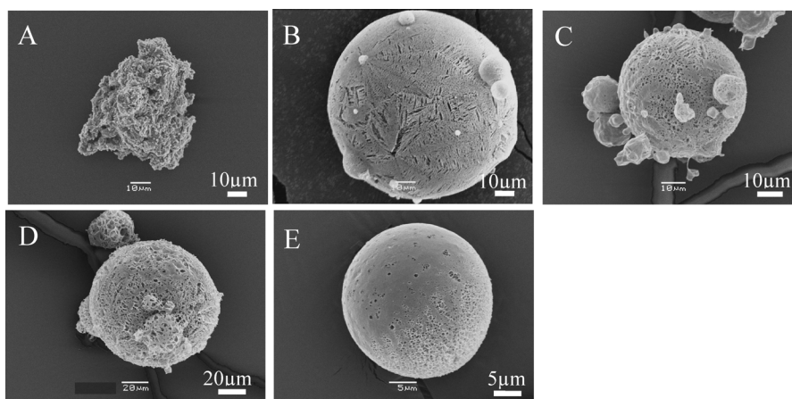
Fig. 5. SEM Photographs of Samples with Varying Mixture Ratio
