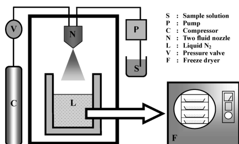
Fig. 1. Schematic Diagram of Spray Freeze Drying (SFD) Apparatus with Two-Fluid Nozzle
