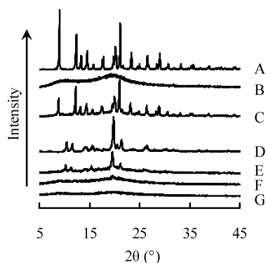
Fig. 6. Powder X-Ray Diffraction Patterns of Samples
