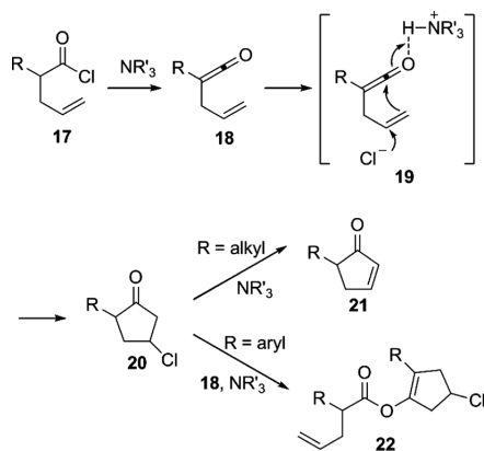
Chart 1. Proposed Mechanism for Trialkylamine-Promoted Intramolecular Acylation of Alkenes with Carboxylic Acid Chlorides
