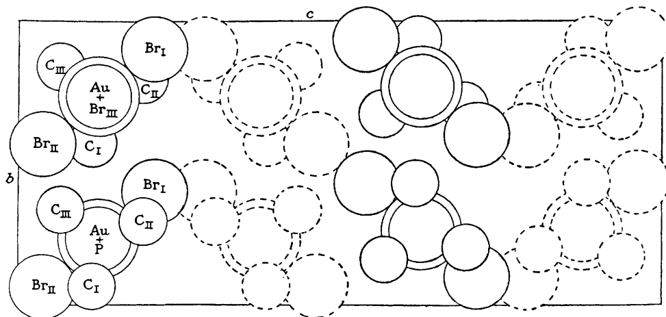
Unit cell projected on (100). Full circles represent atoms at the height x , dashed circles represent atoms at x + \frac{1}{2} . The molecules are here seen end-on, with the Br III 's in the top layer and the phosphine groups in the bottom layer pointing towards the observer. (1 cm. = 2 Å.)
