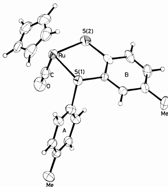
FIGURE. Molecular structure of [Ru(CO)(SC_6H_3Me-o-SC_6H_4Me)(\eta-C_5H_5)] ( 2d ).
