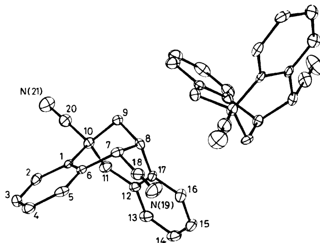
FIGURE. X-Ray structure of compound (5) showing the two independent molecules in the asymmetric unit.
