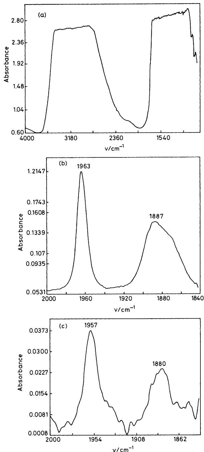
Figure 1. Fourier transform i.r. spectra: †(a) lamb uterine cytosol (micropellet of the lyophilized precipitate); (b) compound (5) in \text{CHCl}_3 ; expansion of the metal carbonyl region; (c) lamb uterine cytosol incubated with compound (5), following base-line correction and subtraction of the spectrum in (a).
