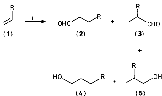
Scheme 1. i, \text{H}_2/\text{CO}, [\text{M}^0] (M = Rh, Co).
