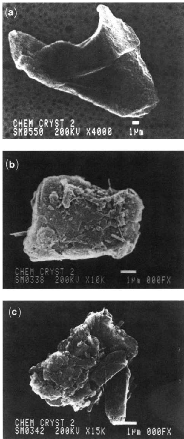
Figure 1. The effect of ultrasonic irradiation on particle morphology: TaS 2 . (a) Before u.s., ~60 μm; (b) 10 min u.s., ~7 μm; (c) 120 min u.s., ~5 μm.
