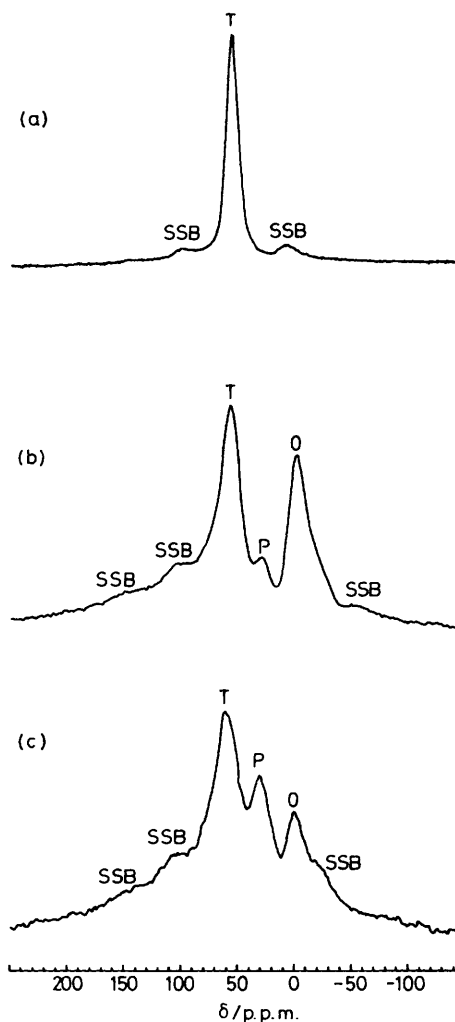
Figure 1. 27 Al N.m.r. spectra of steamed amorphous SiO 2 -Al 2 O 3 . (a) Sample A [T (tetrahedral) 56.2, O (octahedral) + SSB (spinning side band) 8.5 p.p.m.]. (b) Sample B [T 57.9, P (penta-co-ordinated) 28.8, O -0.8 p.p.m.]. (c) Sample F (T 59.6, P 29.1, O -1.3 p.p.m.).
