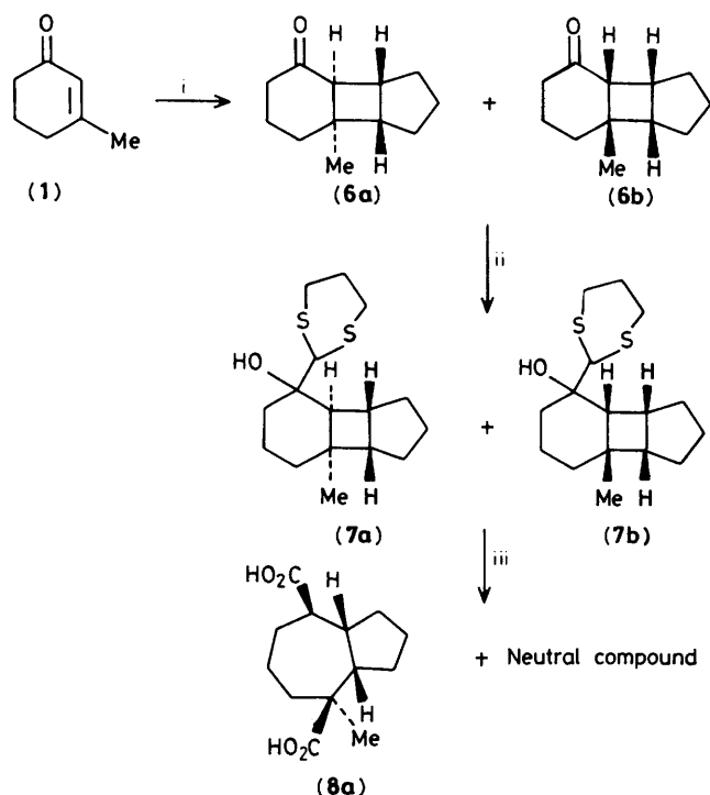
Scheme 2. Reagents and conditions: i, cyclopentene, hν , cyclohexane, -10^{\circ}\text{C} , 5 h, 92%; ii, 1,3-dithiane, \text{Bu}^n\text{Li} , THF, -10^{\circ}\text{C} , 87%; iii, \text{HgO} (red), \text{HBF}_4 (48%), aq. THF (15%), room temp., 2 h, Jones reagent, 0^{\circ}\text{C} , 48%.
