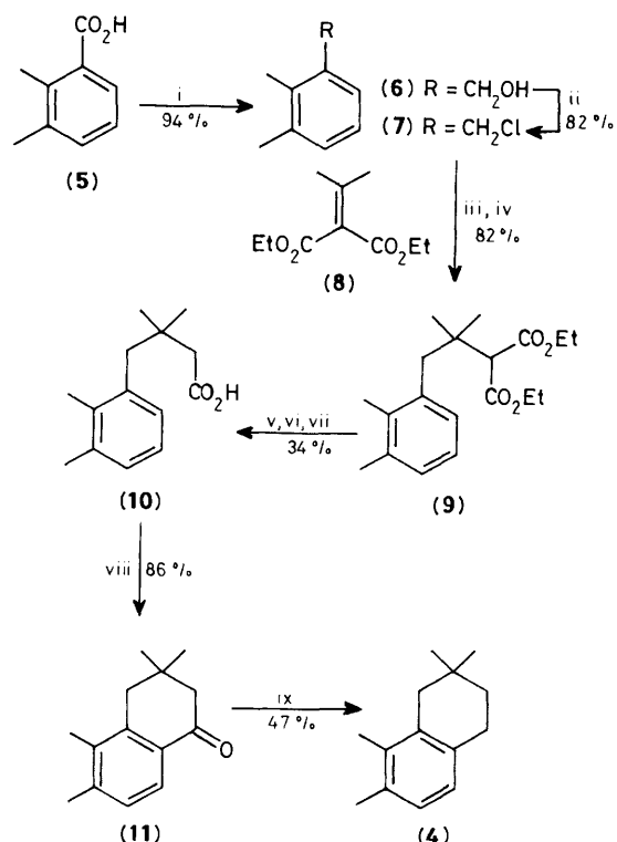
Scheme 1. Reagents and conditions. (i) \text{LiAlH}_4 , ether, reflux; (ii) \text{HCl} , dry hexane, 0^\circ\text{C} ; (iii) \text{Mg} , ether, \text{BrCH}_2\text{CH}_2\text{Br} ; (iv) ( 8 ), ether, 20^\circ\text{C} , 2 h; (v) \text{KOH} , \text{H}_2\text{O} reflux, 3 h; (vi) \text{H}_2\text{SO}_4 , \text{H}_2\text{O} ; (vii) 120^\circ\text{C} , 1.5 h; (viii) \text{PCl}_5 , \text{SnCl}_2 ; (ix) \text{NH}_2\text{NH}_2 , \text{KOH} , diethylene glycol, reflux.
