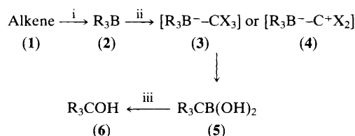
Scheme 1. Reagents and conditions: i, \text{BH}_3\text{-SMe}_2 in benzene (or THF); ii, \text{CHCl}_3 , aq. \text{NaOH} ; iii, \text{H}_2\text{O}_2 .
