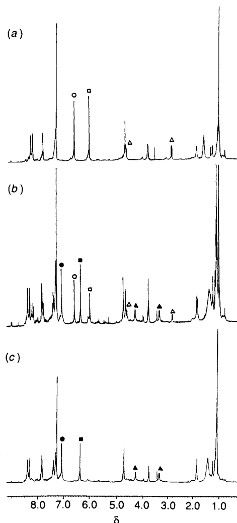
Fig. 1 1 H NMR spectra of the fluorescent calix[4]arene I in CDCl 3 at 25 °C. (a) R = [\text{NaSCN}]/[\text{I}] = 0 , (b) R = 0.5 , (c) R = 1 , where [\text{I}] = 5.1 mmol dm -3 . Aliquots from CD 3 OD solution of 1 mol dm -3 NaSCN were added directly to a CDCl 3 solution of I in an NMR tube; (O, ● = ArH; Δ, ▲ = ArCH 2 Ar; □, ■ = anthracene-CH 2 ).
