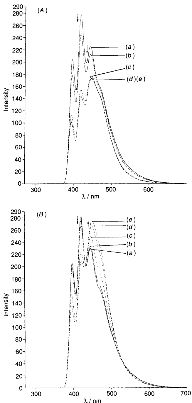
Fig. 2 Fluorescence spectra of I ( 5.00 \times 10^{-6} mol \text{dm}^{-3} ) in chloroform at different concentrations of NaSCN (A) and KSCN (B). [MeSCN] = (a) 0, (b) 1.0 \times 10^{-6} , (c) 4.0 \times 10^{-6} , (d) 6.0 \times 10^{-6} , (e) 8.0 \times 10^{-6} mol \text{dm}^{-3} . The spectra were measured with excitation at 388 nm.
