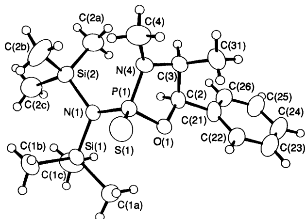
Fig. 1 Structure of \{O,N-(1R,2S)\text{-OCHPhCHMeNMe}\}P(=S)N(\text{SiMe}_3)_2 3. Selected distances (Å) and angles ( ^\circ ): S(1)–P(1) 1.931(2), N(1)–P(1) 1.654(3), N(4)–P(1) 1.661(3), O(1)–P(1) 1.604(2); P(1)–N(1)–Si(1) 116.86(14), P(1)–N(1)–Si(2) 119.91(14), Si(1)–N(1)–Si(2) 120.8(14), C(4)–N(4)–P(1) 122.5(3), C(3)–N(4)–P(1) 111.4(2), C(4)–N(4)–C(3) 117.8(3).
