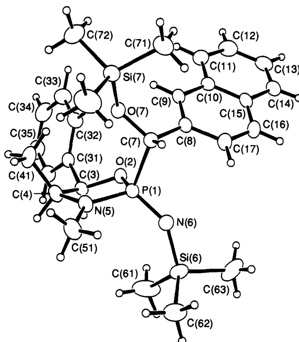
Fig. 2 Structure of \{O,N-(1R,2S)\text{-OCHPhCHMeNMe}\}P(=N\text{-SiMe}_3)\text{C}_{11}\text{H}_8(\text{OSiMe}_3) 6. Selected distances (Å) and angles ( ^\circ ): P(1)–N(6) 1.525(3), P(1)–C(7) 1.841(3), P(1)–N(5) 1.637(3), P(1)–O(2) 1.606(2); P(1)–N(6)–Si(6) 140.8(2), C(7)–O(7)–Si(7) 122.2(2), C(51)–N(5)–P(1) 125.4(2), C(4)–N(5)–P(1) 114.9(2), C(51)–N(5)–C(4) 119.3(3).
