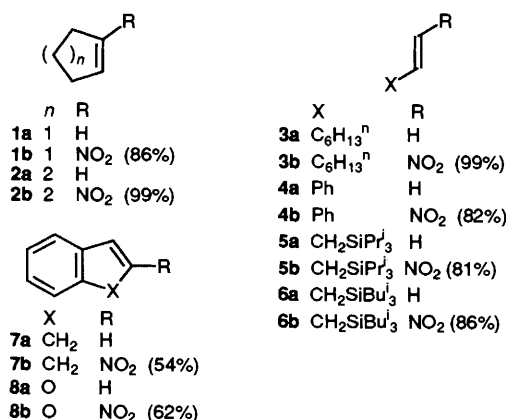
Scheme 1 Sonochemical nitration of alkenes to give the corresponding \alpha,\beta -unsaturated nitroalkenes in a sealed tube by use of the following conditions: NaNO 2 (10 equiv.), Ce(NH 4 ) 2 (NO 3 ) 6 (2.0 equiv.), AcOH, chloroform; 25–73 °C; 4 h
