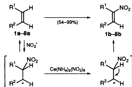
Scheme 1 Sonochemical nitration of alkenes to give the corresponding \alpha,\beta -unsaturated nitroalkenes in a sealed tube by use of the following conditions: NaNO 2 (10 equiv.), Ce(NH 4 ) 2 (NO 3 ) 6 (2.0 equiv.), AcOH, chloroform; 25–73 °C; 4 h
