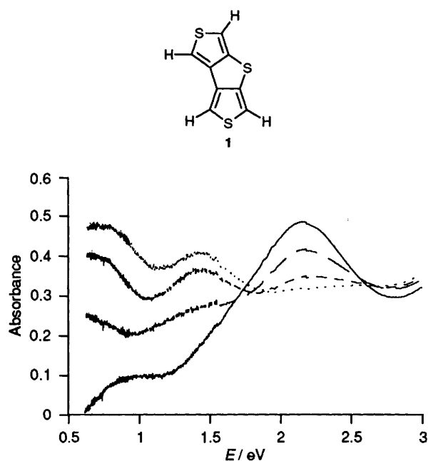
Fig. 1 Electron absorption spectra of PDTT film recorded in situ during the electrochemical doping. (—) neutral, (---) light doped, (— — —) doped, (· · · · ·) full doped.
