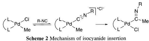
Scheme 2 Mechanism of isocyanide insertion
