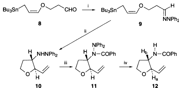
Scheme 3 Reagents and Conditions: i, \text{Ph}_2\text{NNH}_2\cdot\text{HCl} , \text{Et}_3\text{N} , \text{CH}_2\text{Cl}_2 , room temp., 87%; ii, \text{TiCl}_2(\text{OPr})_2 , \text{CH}_2\text{Cl}_2 , -78\text{ }^\circ\text{C} , 82%; iii, BuLi, THF, -78\text{ }^\circ\text{C} , then (\text{PhCO})_2\text{O} , -78\text{ }^\circ\text{C} to room temp., 82%; iv, \text{Sml}_2 , HMPA, THF, room temp., 45%
