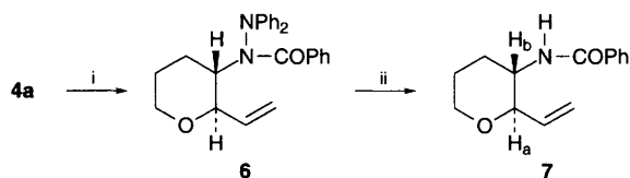
Scheme 2 Reagents and conditions: i, BuLi, THF, -78\text{ }^\circ\text{C} , then (\text{PhCO})_2\text{O} , -78\text{ }^\circ\text{C} to room temp., 83%; ii, \text{Sml}_2 , HMPA, THF, room temp., 98%
