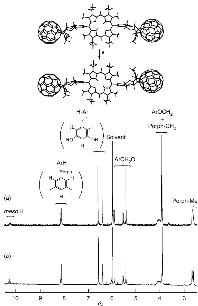
Fig. 1 ^1\text{H} NMR spectra of 1 ( \text{CDCl}_2\text{CDCl}_2 , 400 MHz) at (a) 125 and (b) 25 °C, and molecular models of the two conformers of compound 1 (the four didodecyloxyphenyl groups have been omitted for clarity)
