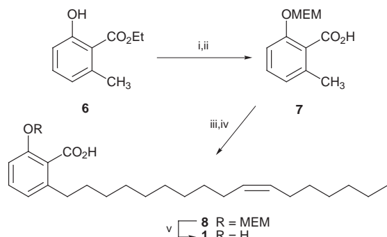
Scheme 1 Reagents and conditions: i, MEMCl, Pr 2 NEt; ii, Bu t OK, 61% over 2 steps; iii, LDA; iv, (9Z)-hexadec-9-enyl bromide, 68% over 2 steps; v, ZnBr 2 , 80%.
