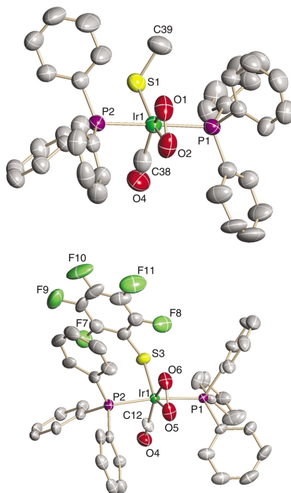
Fig. 1 (Top): ORTEP diagram of the peroxy thiolato complex 3 . Selected bond lengths (Å) and angles (°): O(1)⋯S(1) 3.69, O(1)–O(2) 1.473(3), Ir(1)–C(38) 1.917(7), Ir(1)–S(1) 2.375(2), Ir(1)–O(1) 2.027(2), Ir(1)–P(1) 2.3575(8), Ir(1)–P(2) 2.3563(8); O(1)–Ir(1)–S(1) 116.70(8), C(38)–Ir(1)–S(1) 92.2(2). (Bottom): ORTEP diagram of peroxy thiolato complex 4 . Selected bond lengths (Å) and angles (°): O(6)⋯S(3) 3.55, O(5)–O(6) 1.474(9), Ir(1)–C(12) 1.891(9), Ir(1)–S(3) 2.436(3), Ir(1)–O(5) 2.2029(6), Ir(1)–O(6) 2.017(6), Ir(1)–P(1) 2.388(3), Ir(1)–P(2) 2.400(3); O(6)–Ir(1)–S(3) 105.2(3), C(12)–Ir(1)–S(3) 92.4(8).
