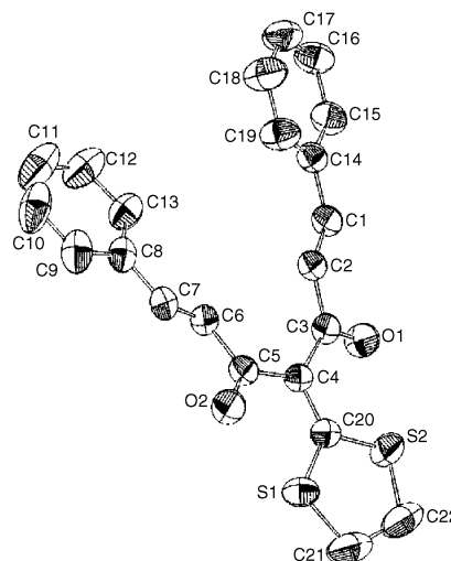
Fig. 1 ORTEP drawing of 4-(1,3-dithiolan-2-ylidene)-1,7-diphenyl-1,6-heptadiene-3,5-dione 2a .
