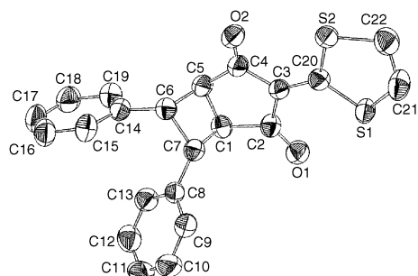
Fig. 3 ORTEP drawing of 3-(1,3-dithiolan-2-yliden)-6,7-diphenylbicyclo[3.2.0]heptane-2,4-dione 3a .
