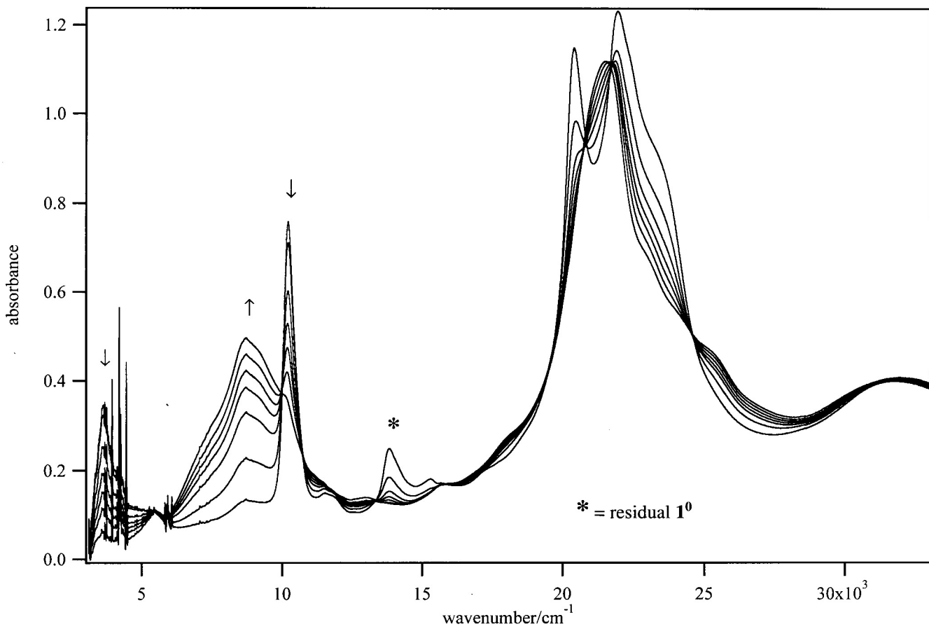
Fig. S3: OTTLE cell progression in the reduction of 1^- to 1^{2-}
