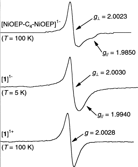
Fig. S4. EPR spectra measured in situ.
