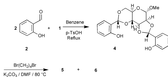
Scheme 2 Alternative synthetic path of polycondensation.
