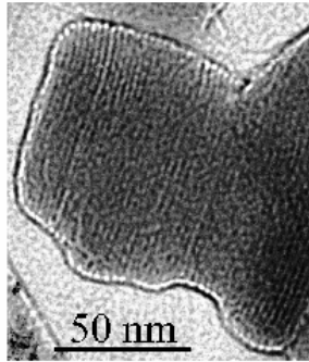
Fig. Transmission Electron Micrograph of Mg 2 Al(OH) showing the layered structure.
