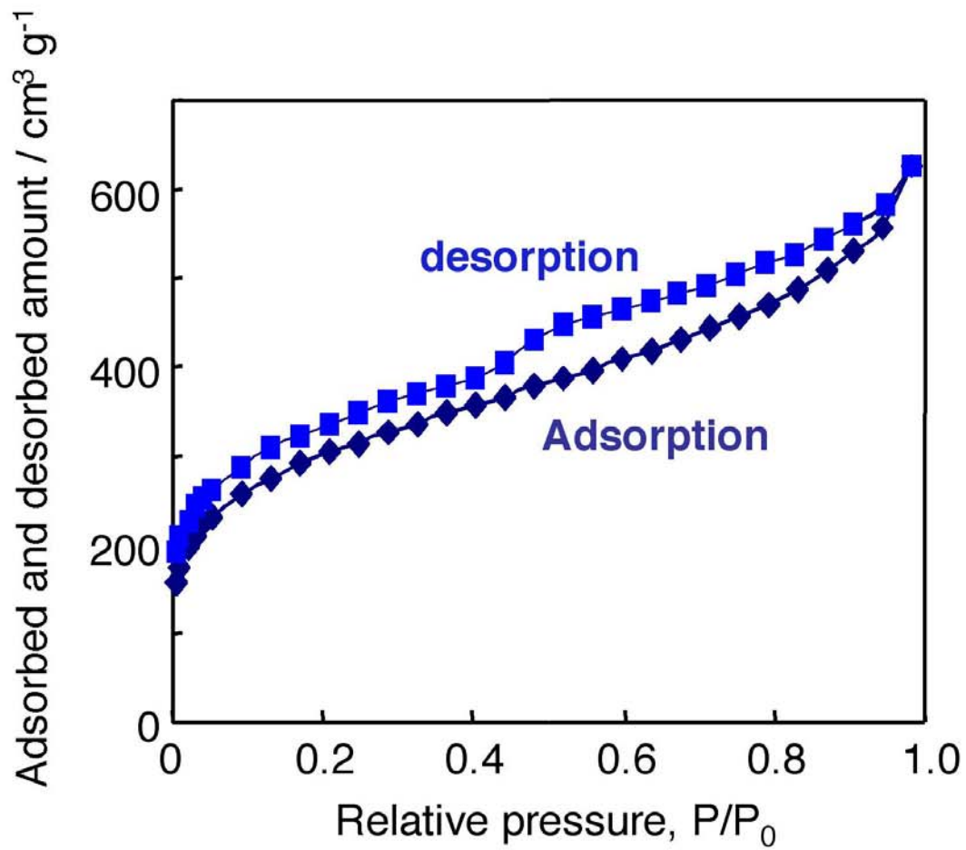
Figure Adsorption-desorption isotherms of N 2 at 77 K
