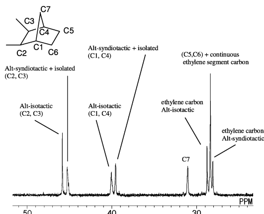
Fig. 1 ^{13}\text{C} NMR spectrum for the ethylene/NB copolymer prepared by complex 2 /MAO (entry 2).
