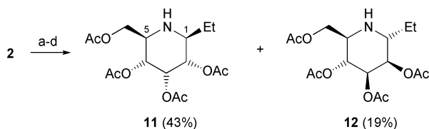
Scheme 3 Reagents and conditions: (a) \text{BF}_3 \cdot \text{Et}_2\text{O} , \text{Et}_2\text{Zn} , \text{CH}_2\text{Cl}_2 , -20^\circ\text{C} \rightarrow \text{rt} , 2 h; (b) \text{OsO}_4 (cat.), N -methylmorpholine N -oxide, acetone– \text{H}_2\text{O} , 5 d; (c) \text{Ac}_2\text{O} , pyridine, 2 h; (d) piperidine, \text{CH}_2\text{Cl}_2 , 1 h.
