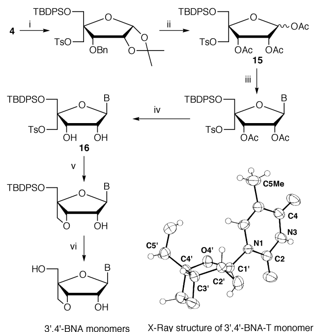
3',4'-BNA monomers X-Ray structure of 3',4'-BNA-T monomer
