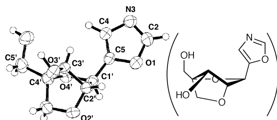
X-Ray structure of 2',4'-BNA C -nucleoside (Ar = oxazol-5-yl)
