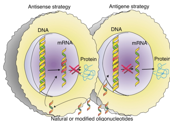
Fig. 2 Representation of antisense and antigene strategies.
