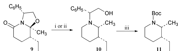
Scheme 2 Reagents and conditions: i, Red-Al, THF, reflux, 8 h, 60%; ii, \text{AlH}_3 , THF, -78^\circ\text{C} , 90 min, then 25^\circ\text{C} , 2 h, 84%; iii, \text{H}_2 , \text{Pd}(\text{OH})_2/\text{C} , (\text{Boc})_2\text{O} , \text{AcOEt} , 25^\circ\text{C} , 82%.
