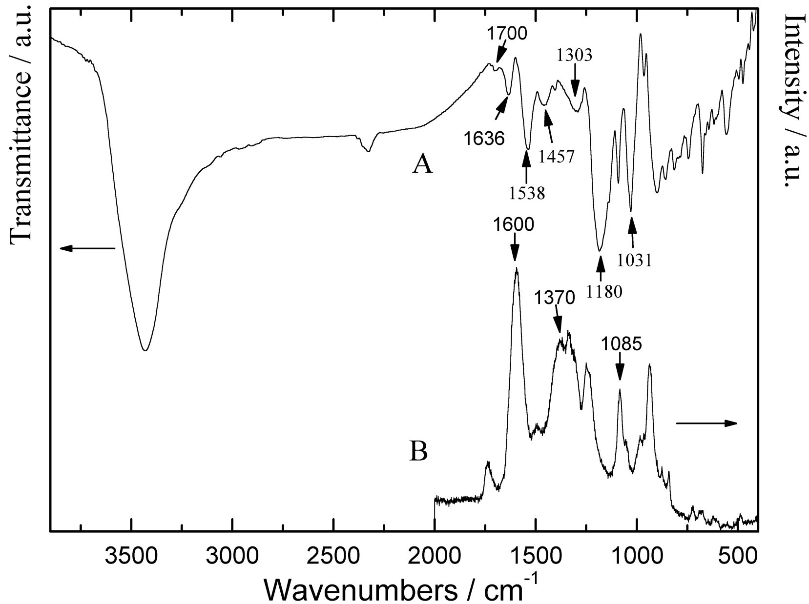
Figure (supplement). The transmittance infrared (A) and 633 nm excited Raman spectrum (B) of a PPy film with microcups generated at a constant potential of 1.2 V (vs SCE)
