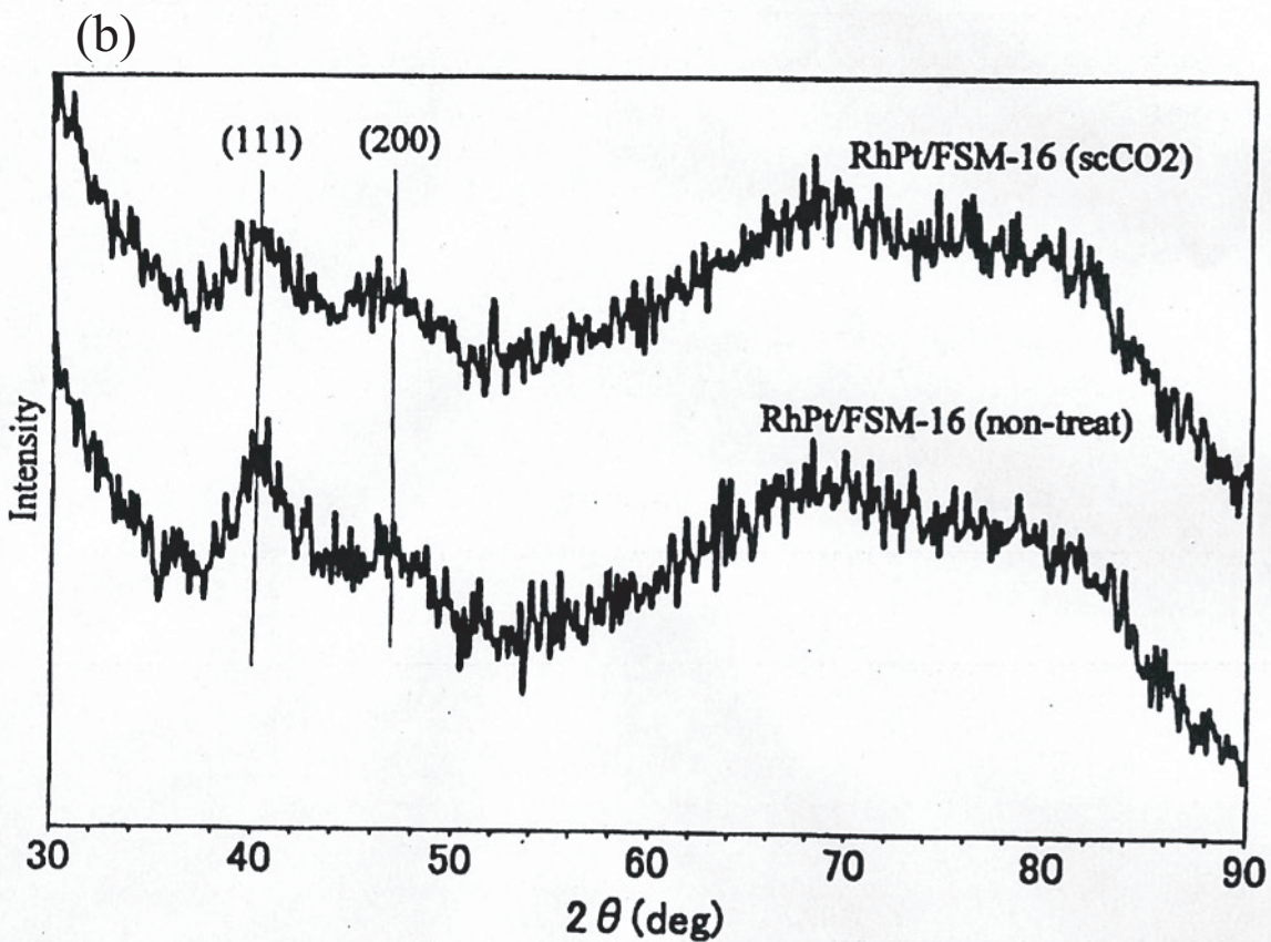
Figure 1s. XRD patterns for RhPt/FSM-16 catalysts: (a) low angle region (b) high angle region
