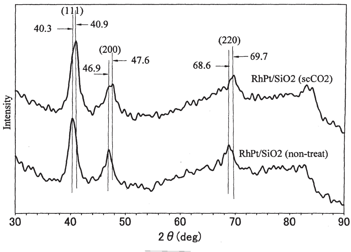
Figure 2s. XRD Patterns for RhPt/SiO 2 catalysts
