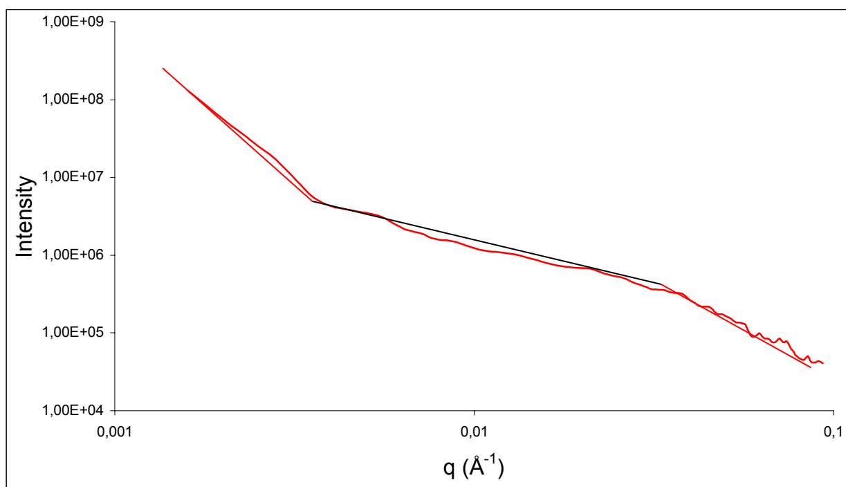
SAXS pattern of material XCu .
