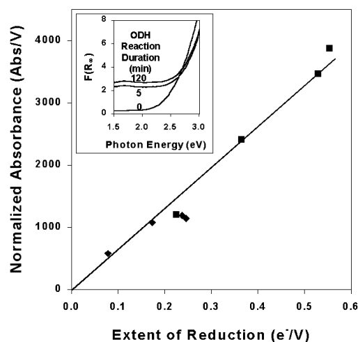
Fig. 1 UV-visible reduction response calibration curve for VO x /Al 2 O 3 catalysts [20 kPa H 2 , balance He, 603 K reduction followed by 5 kPa O 2 , balance He, 298–773 K reoxidation]; ◆: 3.5 wt% V 2 O 5 /Al 2 O 3 , ■: 10 wt% V 2 O 5 /Al 2 O 3 . Inset: UV-visible spectra for 10 wt% V 2 O 5 /Al 2 O 3 [603 K, 14 kPa C 3 H 8 , 1.7 kPa O 2 , balance He].
